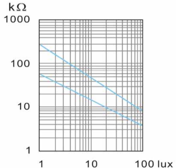
Luminance VS Photo Resistance
